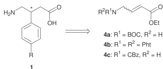
Scheme 1. Strategy for the synthesis of GABA derivatives.
